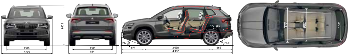
The technical drawings apply to car with petrol engine or 1.6 TDI.
